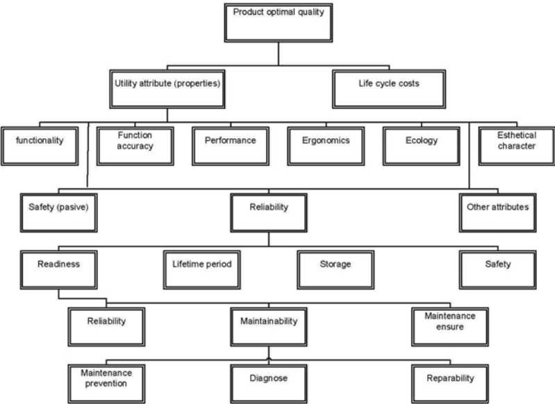
Figure 2. Criterion for evaluate the machine tool of quality and reliability
